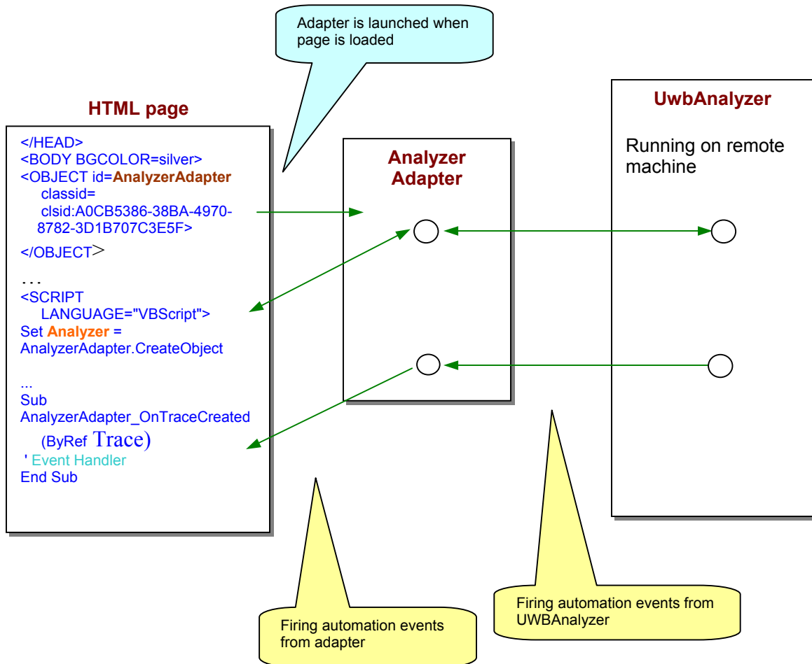
Figure 6-1 Analyzer Adapter
